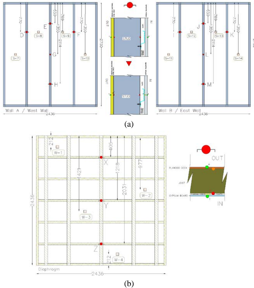
Figure 5. Thermocouple Layout (a) CFS01 Wall (b) WOOD01 Diaphragm
